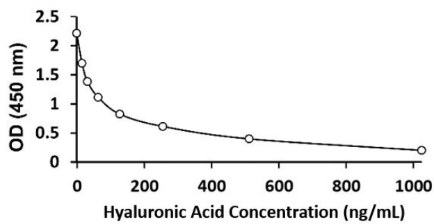
ARG83802 General Hyaluronic Acid ELISA Kit standard curve image
