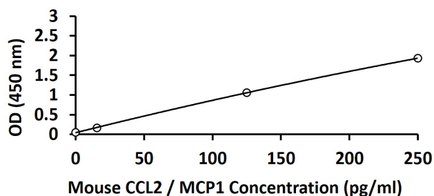
ARG83760 Mouse CCL2 / MCP1 ELISA Kit standard curve image
