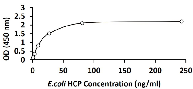
ARG83090 E.coli HCP ELISA Kit standard curve image
