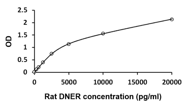
ARG82561 Rat DNER ELISA Kit standard curve image ARG82561 Rat DNER ELISA Kit results of a typical standard run with optical density reading at 450 nm.
