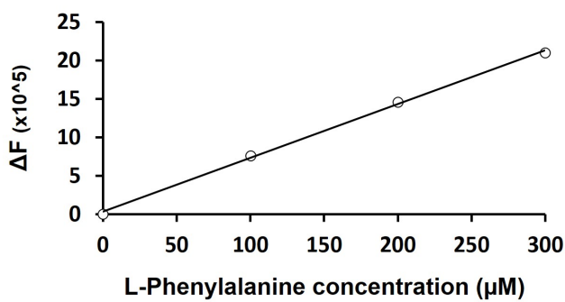
ARG82190 Phenylalanine Assay Kit (Fluorometric) typical data demonstration image
