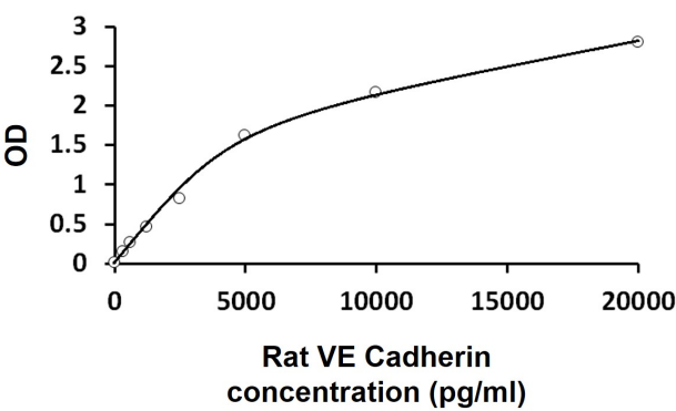
ARG82115 Rat VE Cadherin ELISA Kit standard curve image
