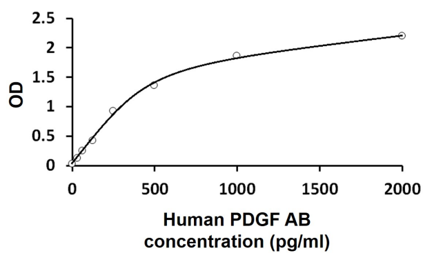
ARG81400 Human PDGF AB ELISA Kit standard curve image
