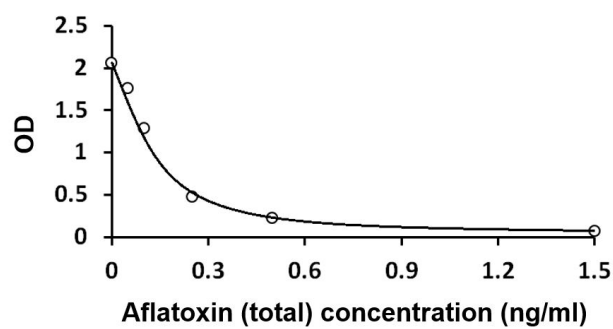
ARG81030 Aflatoxin (total) ELISA Kit standard curve image
