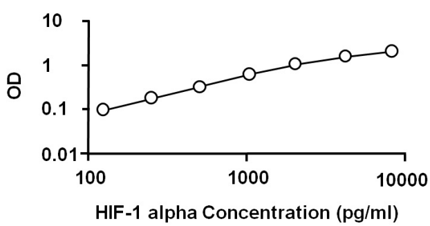
ARG80969 Human/Mouse HIF-1 alpha ELISA Kit standard curve image
