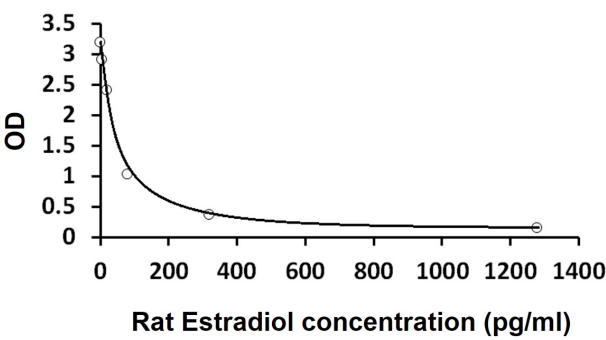
ARG80755 Rat Estradiol ELISA Kit standard curve image
