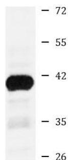
HeLa + Nocodazole
