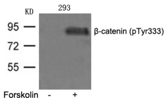
ARG51844 anti-beta Catenin phospho (Tyr333) antibody WB image
