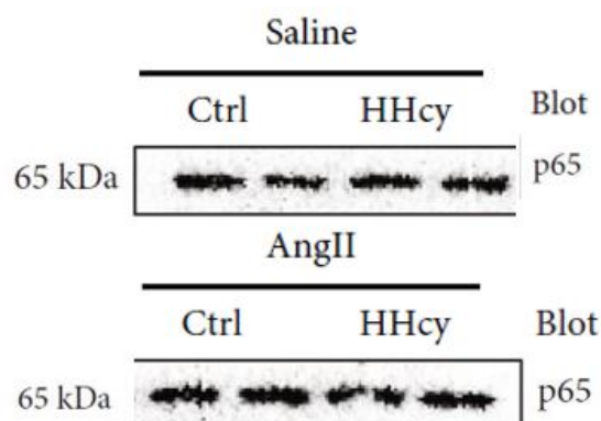
ARG65677 anti-NFκB p65 antibody WB image
